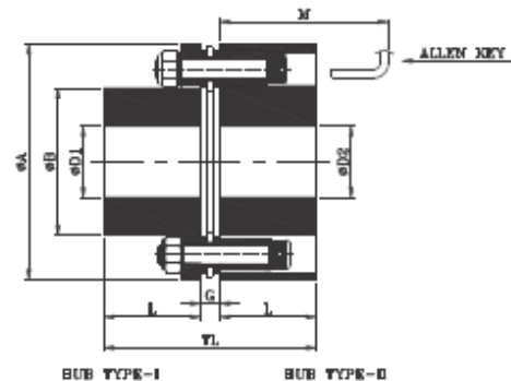
TYPE - RLMK
